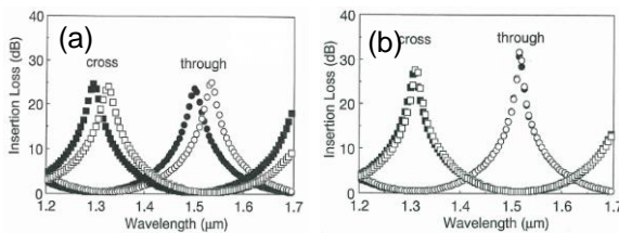
Insertion loss spectra (a) before and (b) after inserting AT-HWP into the waveguide gap.
